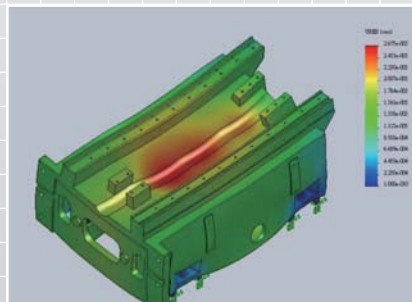
Base displacement analysis
