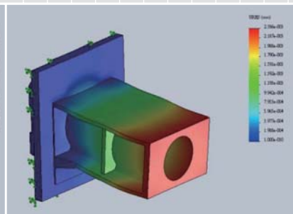
Spindle seat displacement analysis
