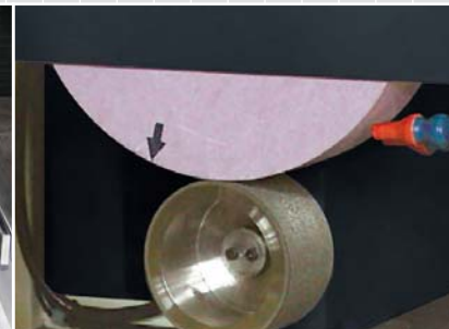
Roller diamond dresser (option)
