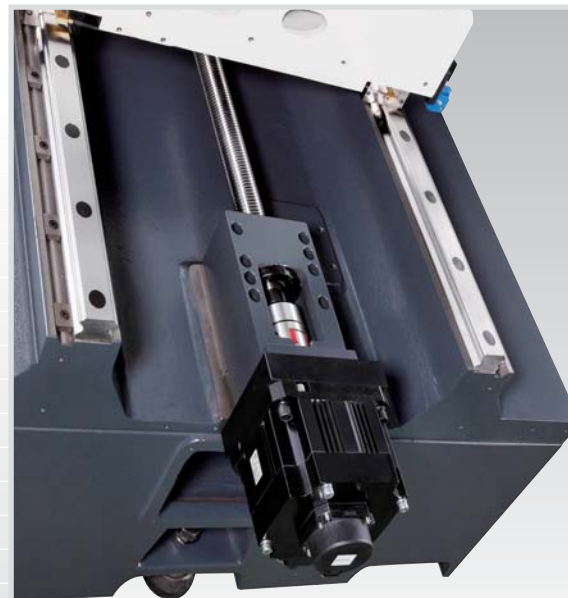
Z axis direct drive transmission mechanism, collocated with super precision Roller type guide way.
