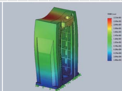
Column displacement analysis
